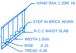
STAIR DETAIL
