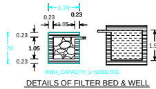
DETAILS OF FILTER BED & WELL
