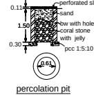
percolation pit
