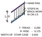
DETAILS OF STAIRCASE
