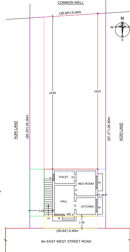
SITE PLAN
