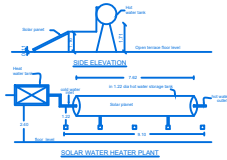
SOLAR WATER HEATER PLANT
