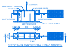
SEPTIC TANK AND U-TRAP ADOPTED
