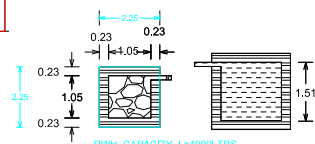
DETAILS OF FILTER BED & WELL
