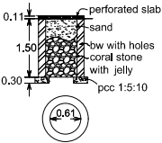
percolation pit
