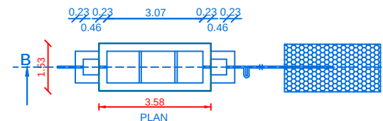
SEPTIC TANK AND TRENCH & U TRAP ADOPTED
