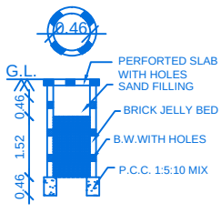
PERCOLATION PIT
