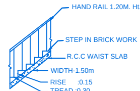
STAIR DETAIL
