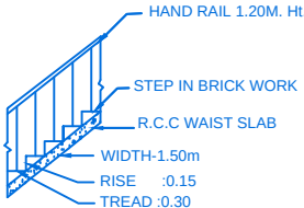
STAIR DETAIL
