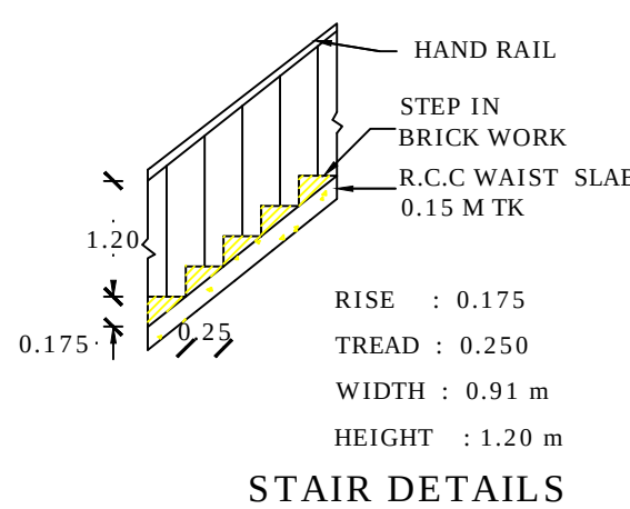
STAIR DETAILS
