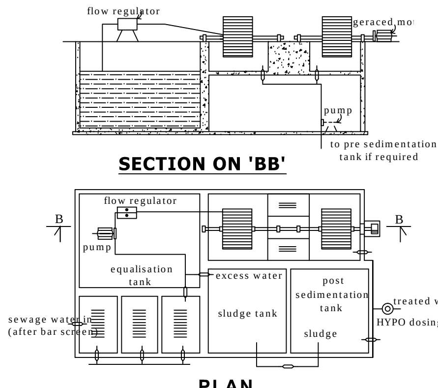
DETAILS OF SEWAGE TREATMENT PLANT
