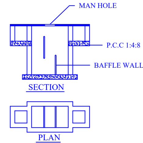
SEPTIC-TANK DETAIL
