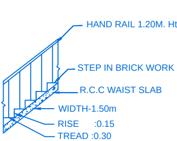
STAIR DETAIL
