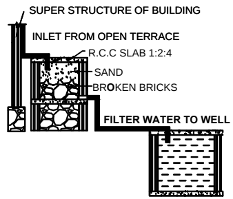
RAINWATER HARVESTING
