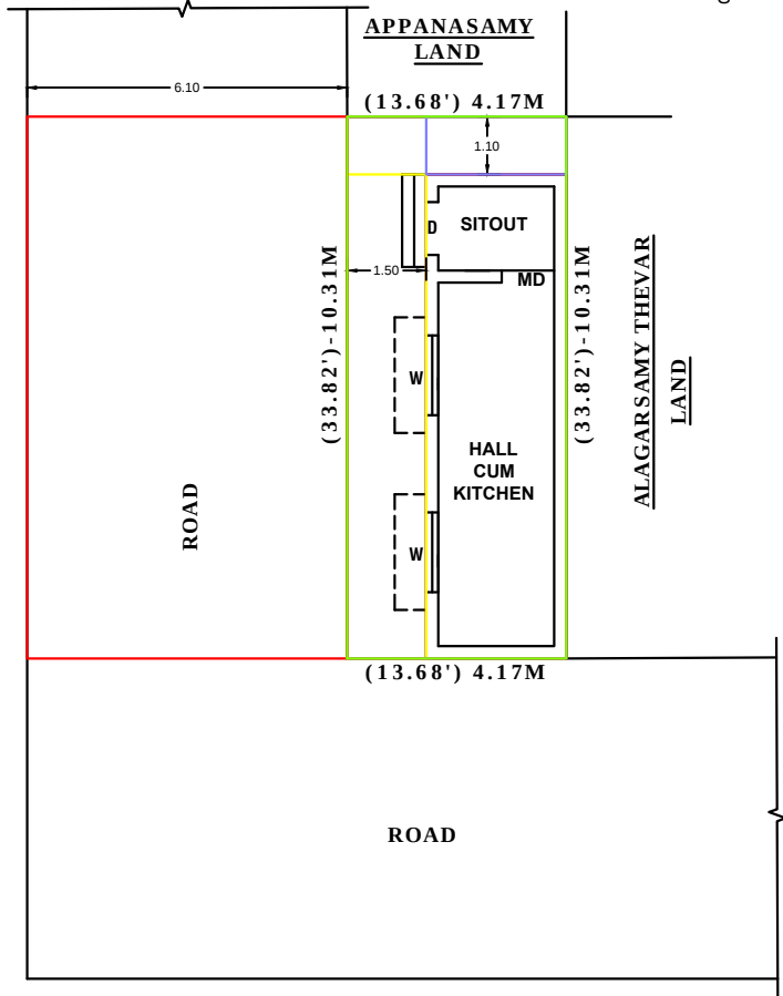
SITE PLAN
