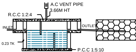
percolation pit
