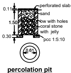
percolation pit
