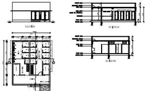
PLAN BLOCK-3
