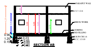
SECTION AB
