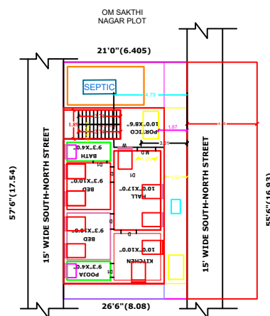
PLOT NO:29 SITE PLAN SCALE 1:100
