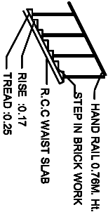
STAIR CASE DETAIL
