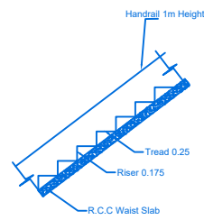
STAIR DETAILS
