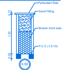
RAIN WATER COLLECTION WELL
