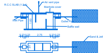
SEPTIC TANK & TRENCH
