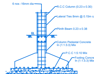
COLUMN FOOTING DETAILS
