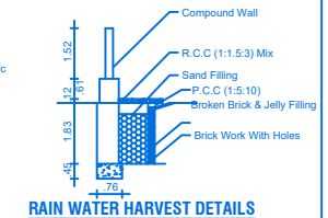
RAIN WATER HARVEST DETAILS
