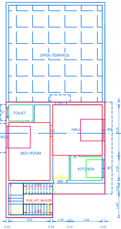
PROP.FIRST FLOOR PLAN
