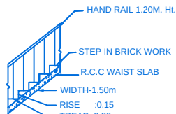
STAIR DETAIL
