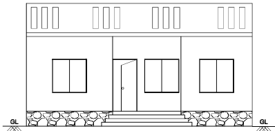
FRONT ELEVATION
