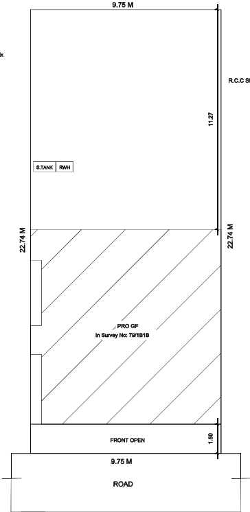
SITE PLAN (1:260)
