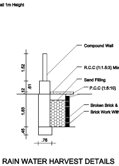
RAIN WATER HARVEST DETAILS
