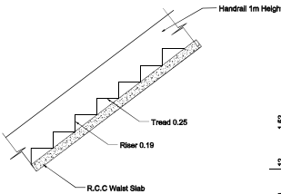
STAIR DETAILS
