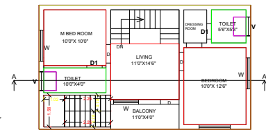
PRO.FIRST FLOOR PLAN
