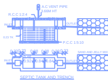
SEWERAGE SYSTEM
