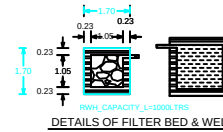
DETAILS OF FILTER BED & WELL
