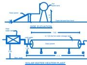
SOLAR WATER HEATER PLAN
