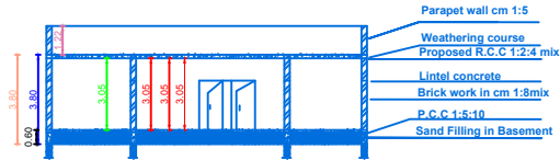
SECTION ON - AB
