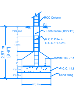
FOUNDATION DETAILS
