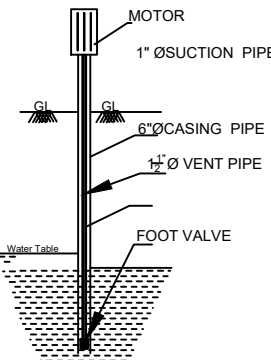
SEC. OF BOREWELL
