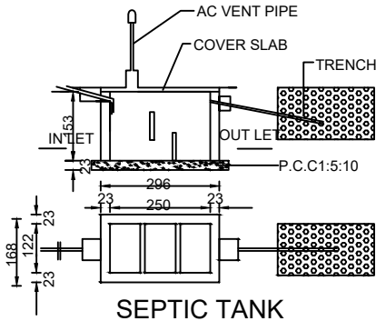
SEPTIC TANK
