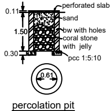
percolation pit
