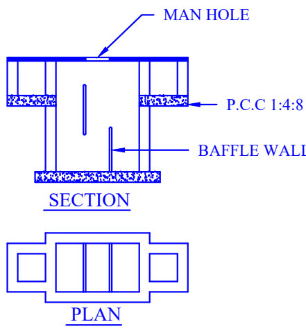
SEPTIC-TANK DETAIL
