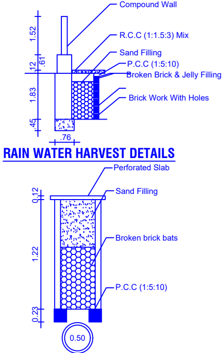
RAIN WATER COLLECTION WELL
