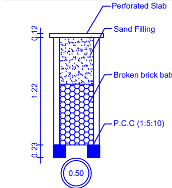
RAIN WATER COLLECTION WELL
