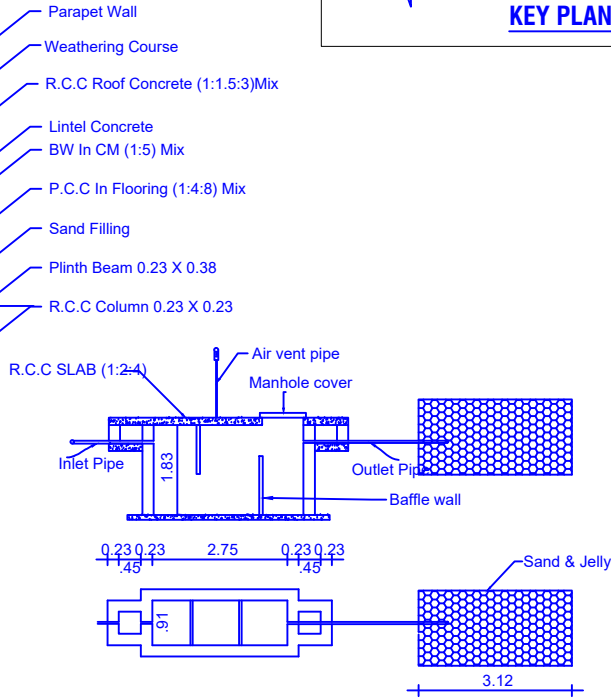
SEPTIC TANK & TRENCH
