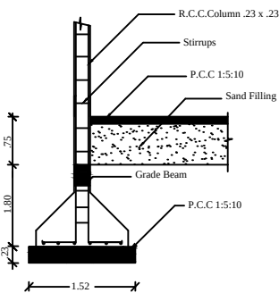
COLUMN DETAIL
