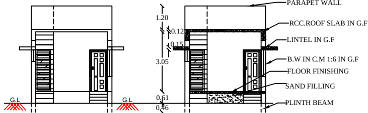
FRONT ELEVATION
