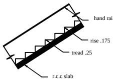
STAIR
