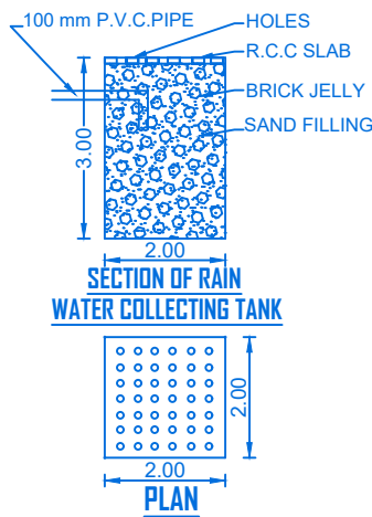
PLAN
