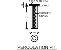
PERCOLATION PIT
