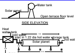
SOLAR WATER HEATER PLANT
