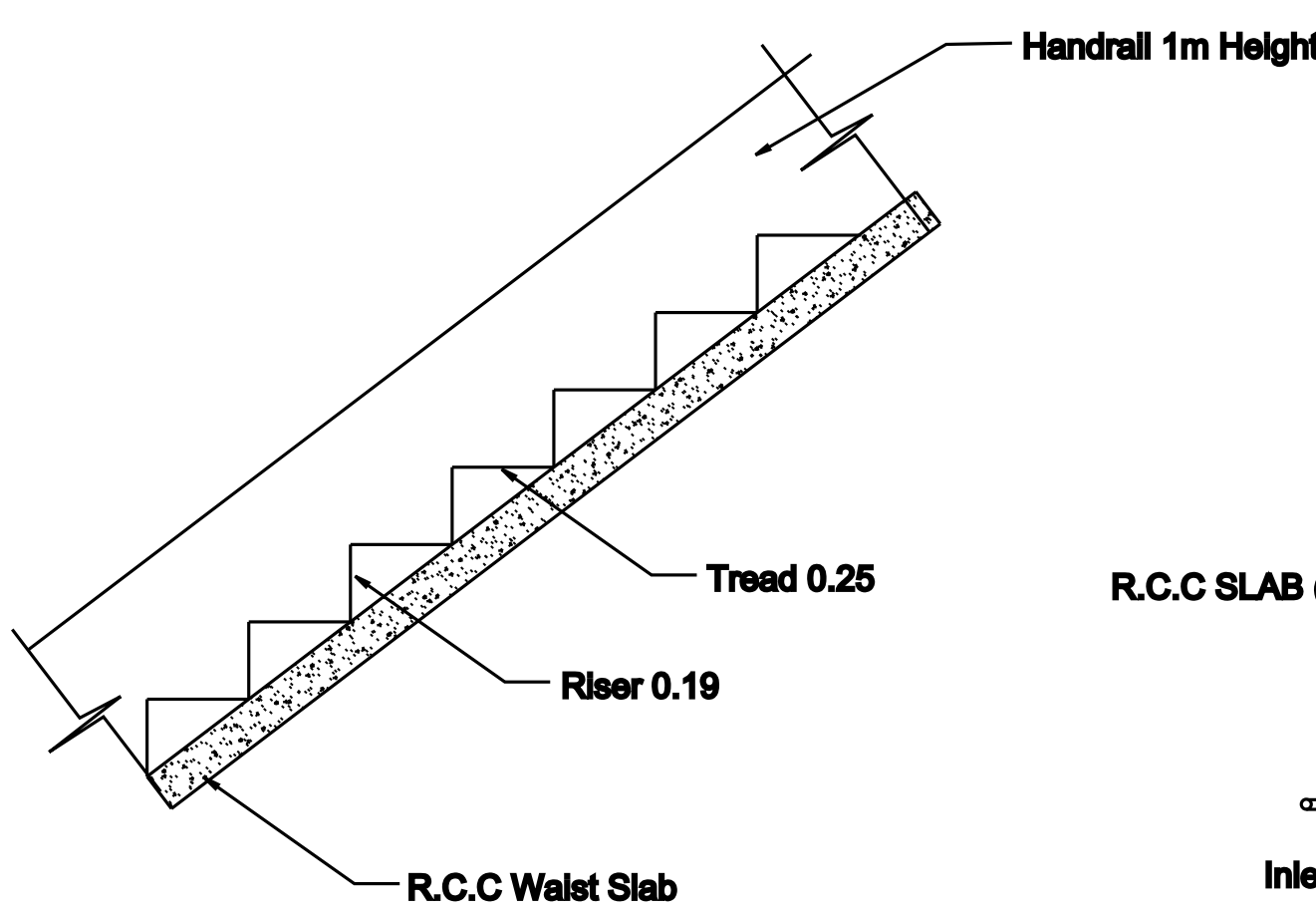
STAIR DETAILS
