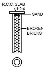
PERCOLATION PIT
