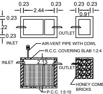
DETAILS OF SEPTIC TANK AND TRENCH
