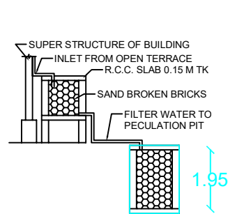
DETAILS OF RAIN WATER HARVESTING
