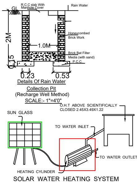
SOLAR WATER HEATING SYSTEM
