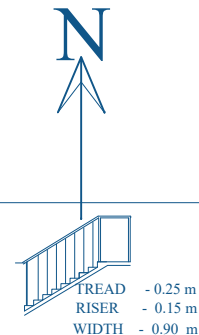
STAIRCASE DETAILS
