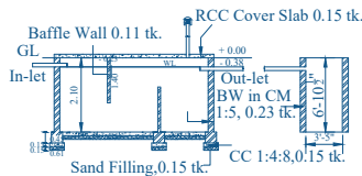
SECTION - SEPTIC TANK
