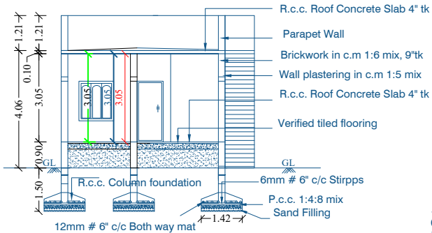
SECTION NN
