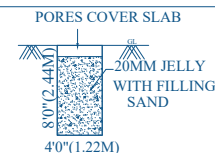
RAINWATER HARVESTING UNIT
