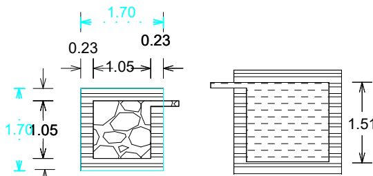
DETAILS OF FILTER BED & WELL
