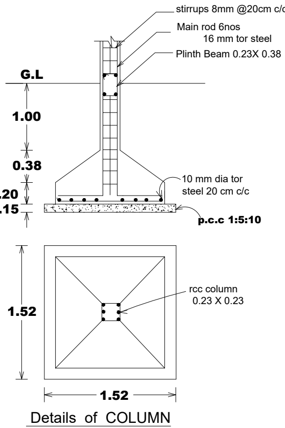
Details of COLUMN
