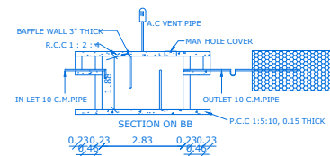
SEPTIC TANK AND TRENCH &amp; U TRAP ADOPTED
