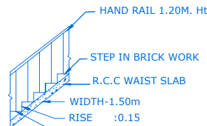
STAIR DETAIL
