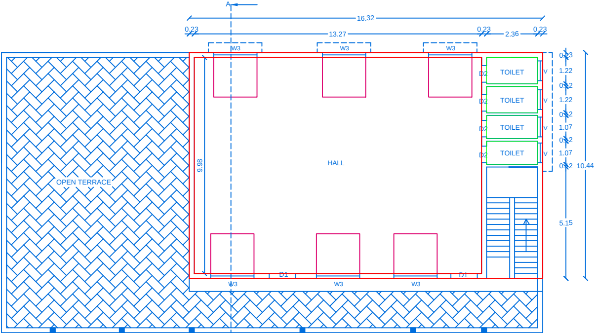
PROP.FIRST FLOOR PLAN
