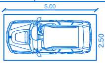
CAR POCKET DETAILS
