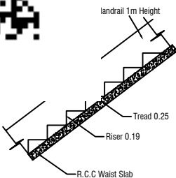
STAIR DETAILS
