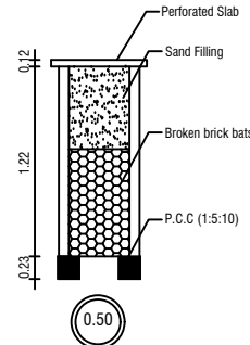
RAIN WATER COLLECTION WELL
