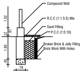
RAIN WATER HARVEST DETAILS
