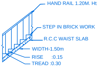
STAIR DETAIL
