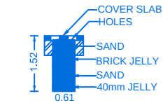
SECTION OF RAIN WATER COLLECTION TANK
