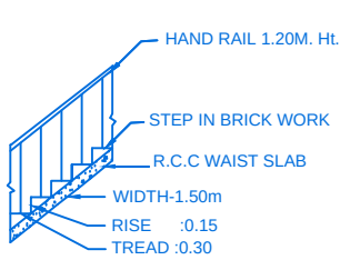
STAIR DETAIL
