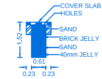
SECTION OF RAIN WATER COLLECTION TANK
