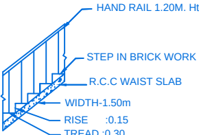
STAIR DETAIL
