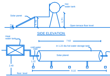
SOLAR WATER HEATER PLANT
