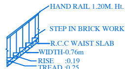
STAIR DETAIL
