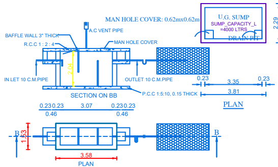
SEPTIC TANK AND TRENCH & U TRAP ADOPTED
