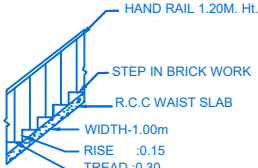
STAIR DETAIL
