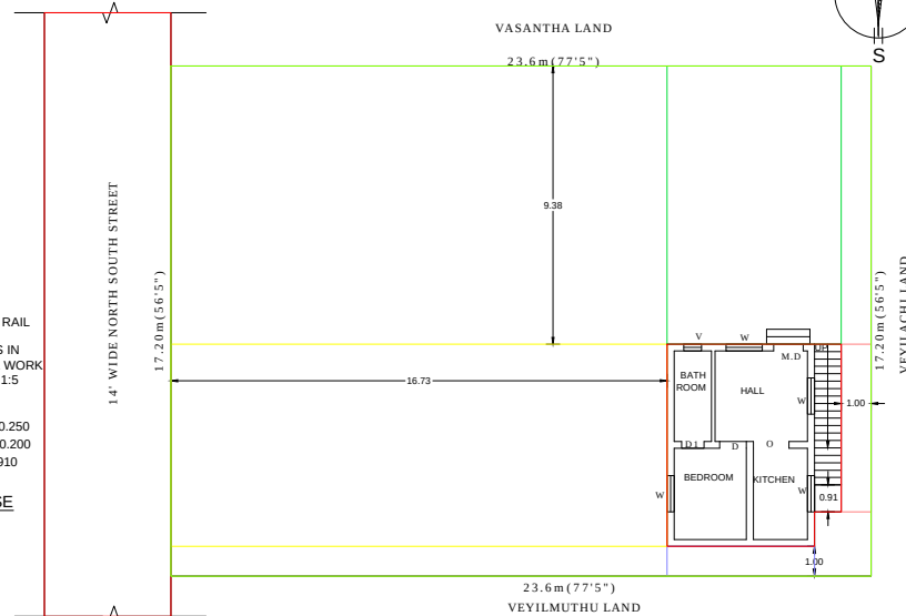
SITE PLAN
