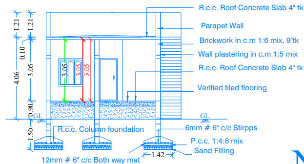
SECTION NN
