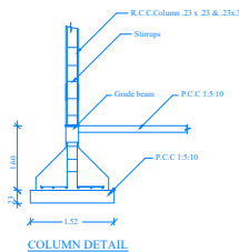
COLUMN DETAIL
