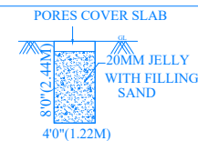
RAINWATER HARVESTING UNIT
