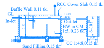
SECTION - SEPTIC TANK
