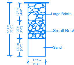
SECTION OF RAIN WATER COLLECTION PITS (NTS)
