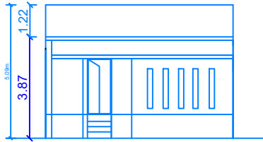
FRONT ELEVATION
