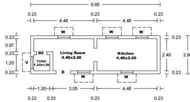
PROPOSED GROUND FLOOR PLAN
