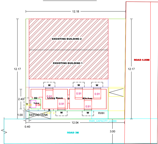
SITE PLAN FOR THE PROPOSAL
