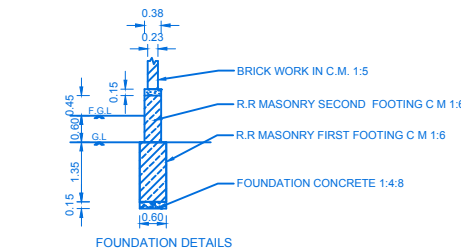
FOUNDATION DETAILS
