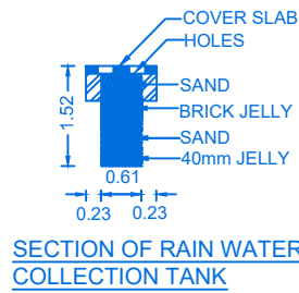
SECTION OF RAIN WATER COLLECTION TANK
