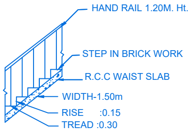
STAIR DETAIL
